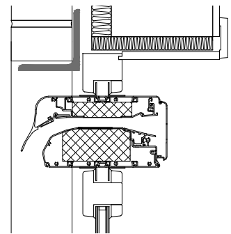
Fully glazed-in (at transom) (recommended installation)
