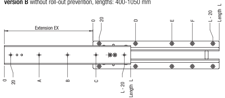
version B without roll-out prevention, lengths: 400-1050 mm
