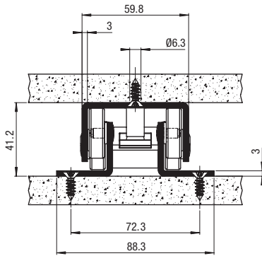
version B without roll-out prevention, lengths: 400-1050 mm
