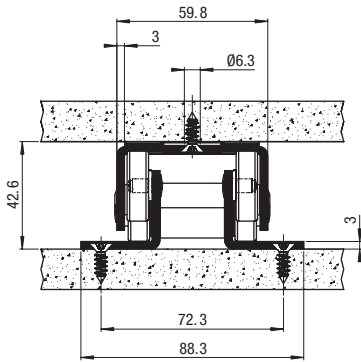
version A with roll-out prevention, lengths: 450-700 mm
