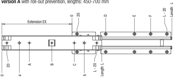
version A with roll-out prevention, lengths: 450-700 mm
