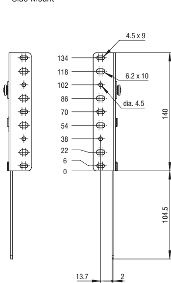
Side Mount
