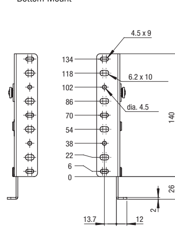
Bottom Mount
