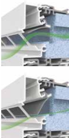
Self-regulating valve
